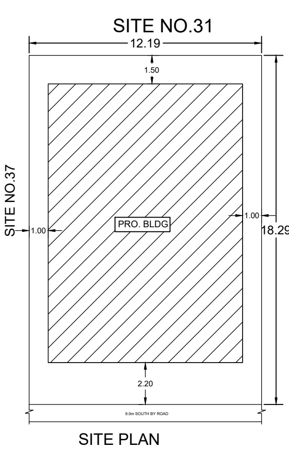
SITE PLAN
